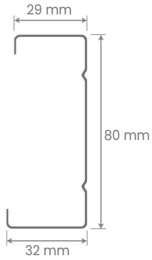
Truss C80 (Motif Diamond)
