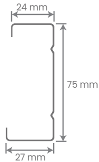
Truss ECO C75 (Motif Diamond)
