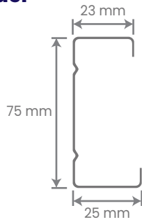
TRUSS ECO C75
