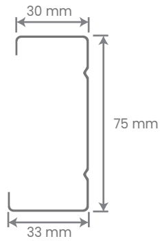
TRUSS C75
